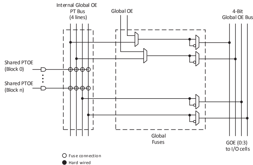
Figure 6.1. Global OE Generation for All Devices Except LA-ispMACH 4032V/Z
