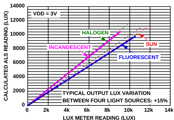
FIGURE 17. LIGHT SENSITIVITY vs LUX LEVEL
