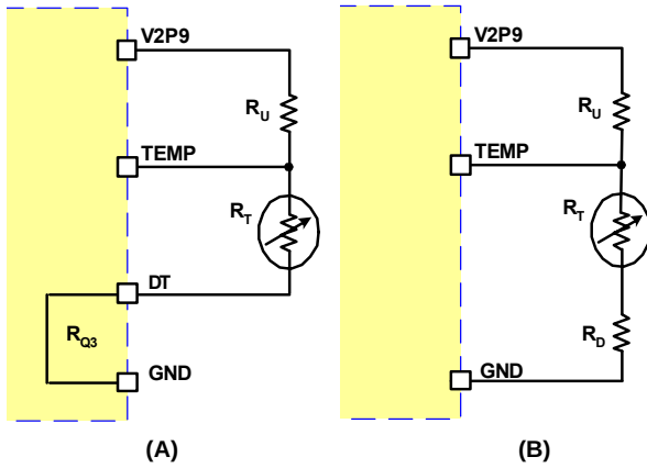
FIGURE 7. EQUIVALENT CIRCUITS FOR THE NTC DIVIDER (A) BEFORE CHARGING STARTS (B) DURING CHARGING.
