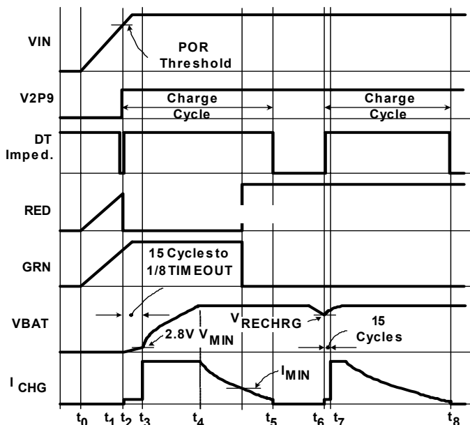
FIGURE 4. OPERATION WAVEFORMS
