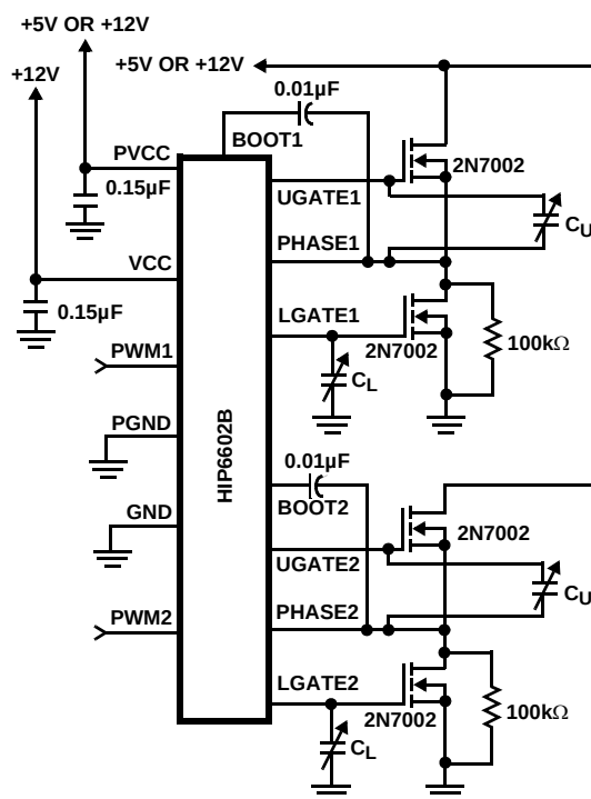
FIGURE 1. HIP6602B TEST CIRCUIT
