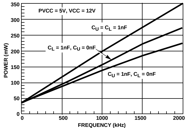
FIGURE 7. POWER DISSIPATION vs FREQUENCY, PVCC = 5V
