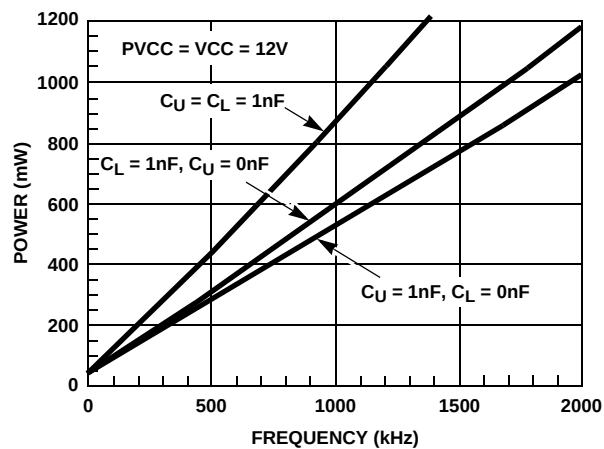
FIGURE 3. 1nF LOADING PROFILE
