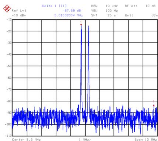
FIGURE 4. TWO TONES (CF=6) AT 8.5MHz, 50MSPS CLOCK, 500kHz SPACING (67dBc - 10MHz WINDOW, 6dB PAD)
