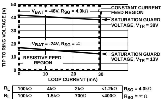
FIGURE 14. V_{TR} vs I_L and R_L
