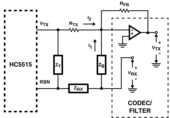
FIGURE 16. TRANSHYBRID CIRCUIT
