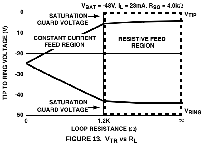
FIGURE 13. V_{TR} vs R_L
