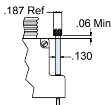
Code E & EJ EJ - Extended Jackscrew E - Extended Screwlock
