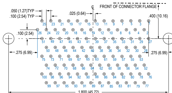
100 SOCKET MWDM-100SCBR
