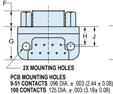
CONFIGURATION FOR 9-25 CONTACTS
