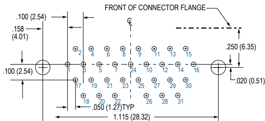
31 PIN MWDM-31PCBR
