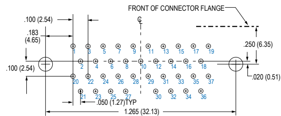
37 PIN MWDM-37PCBR
