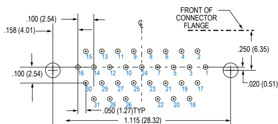
31 SOCKET MWDM-31SCBR
