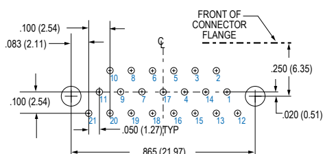
21 SOCKET MWDM-21SCBR
