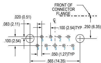
9 SOCKET MWDM-9SCBR
