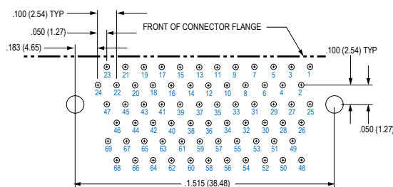
69 SOCKET MWDM-69SCBR
