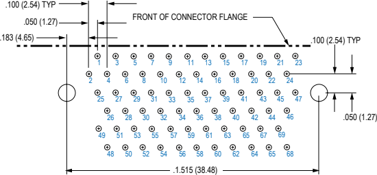
69 PIN MWDM-69PCBR
