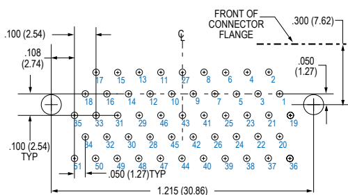
51 SOCKET MWDM-51SCBR
