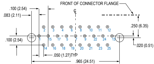
25 PIN MWDM-25PCBR
