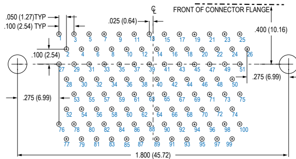
100 PIN MWDM-100PCBR
