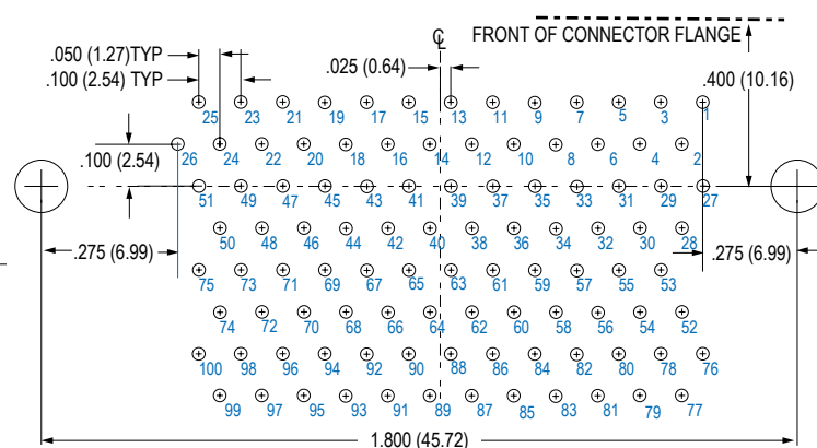
100 SOCKET MWDM-100SCBR
