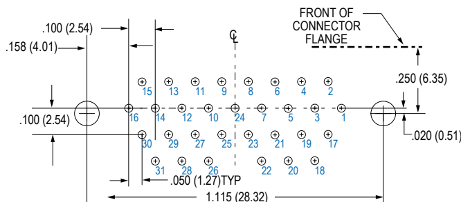
31 SOCKET MWDM-31SCBR
