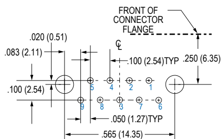
9 SOCKET MWDM-9SCBR
