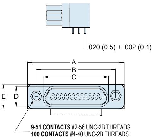
CONFIGURATION FOR 9-25 CONTACTS
