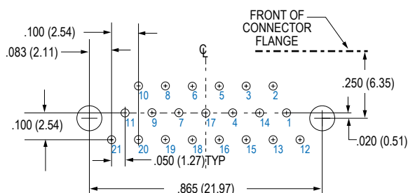
21 SOCKET MWDM-21SCBR
