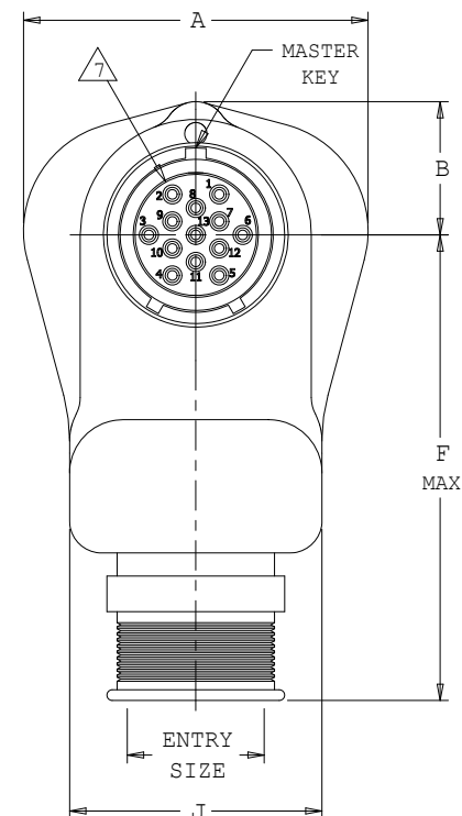
FACE VIEW OF PLUG AS VIEWED FROM ENGAGING END (8-13PA1 SHOWN)
