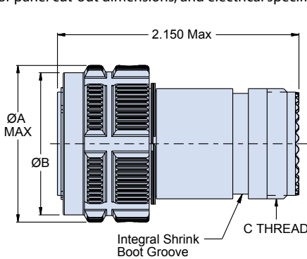
Plug
