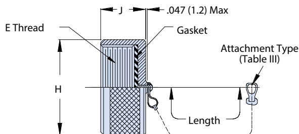
660-005 Receptacle Cover
