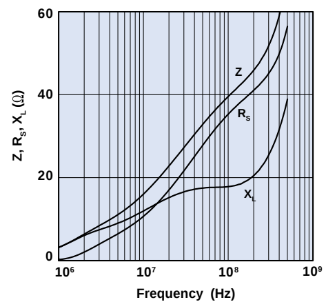
Figure 18 Impedance vs. Frequency for connector EMI suppression plate 2644247101.
