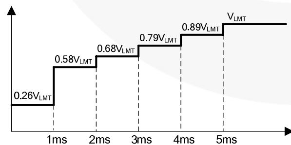
Figure 27. Soft-Start Function
