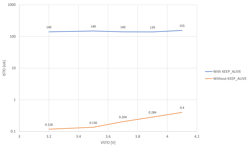
Figure 4: Quiescent current
