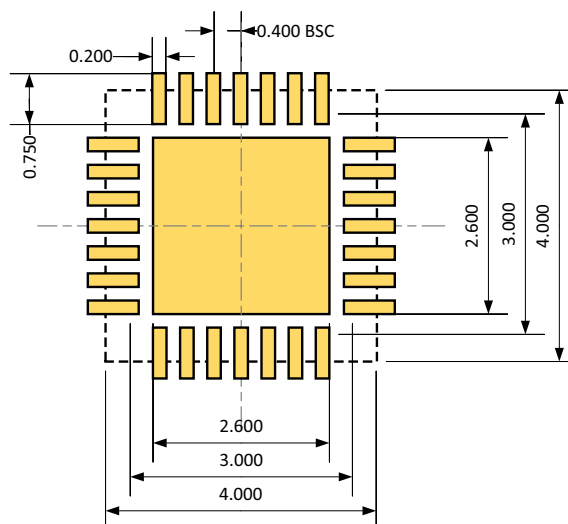
Figure 20: QFN28 4x4 mm board layout
