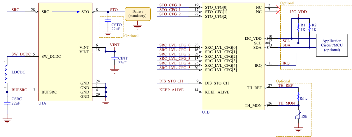
Figure 21: AEM0090x schematic
