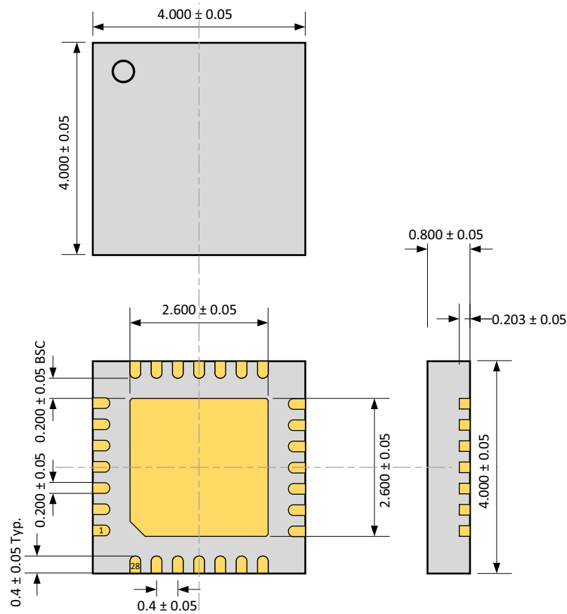
Figure 19: QFN28 4x4 mm
