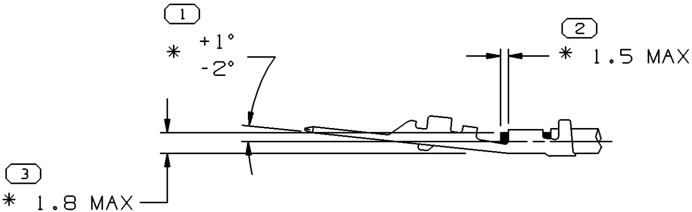
TERMINAL AND CABLE ALIGNMENT SCALE 2:1
