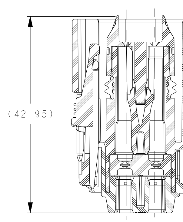
SECTION A - A TPA IN FINAL LOCK POSITION
