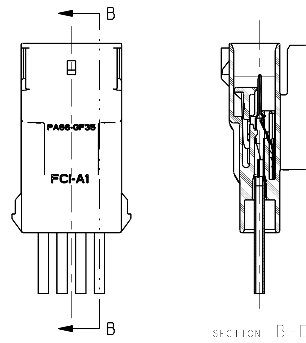
UNSEALED ASSEMBLY VIEW SHORTING CLIP OPTION
