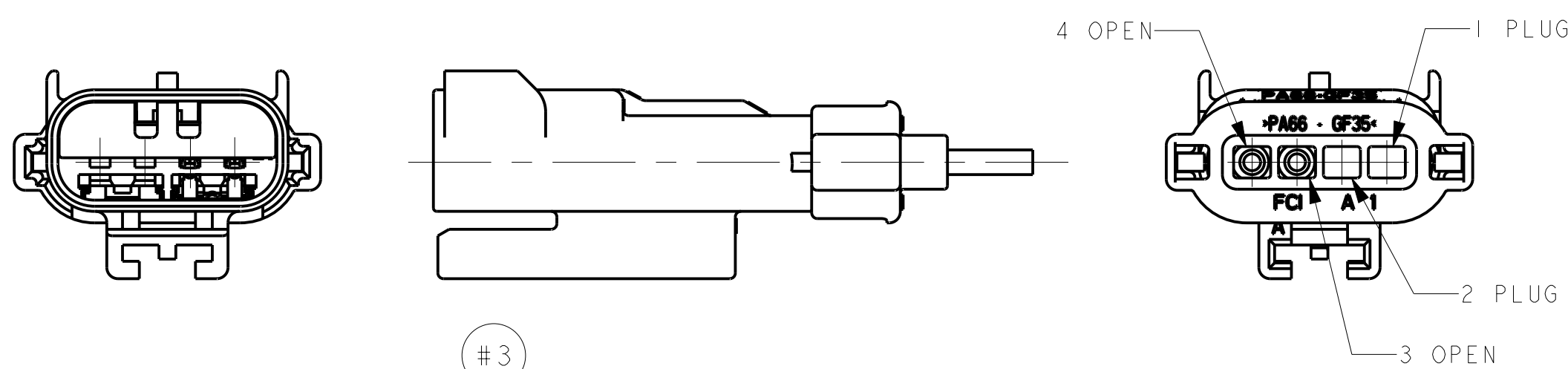
#3 SRS OPTION CIR #1 & 2 PLUGGED CIR #3 & 4 SHORTED/OPEN (UNSEALED ALL CAVITIES OPEN) POL. TYPE "A" SHOWN
