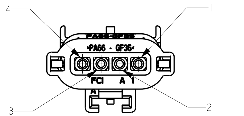
#2 SRS OPTION CIR #1 & 2, 3 & 4 SHORTED/OPEN (UNSEALED ALL CAVITIES OPEN) POL. TYPE "A" SHOWN
