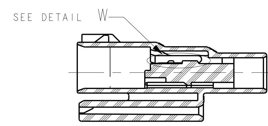
SECTION B-B
