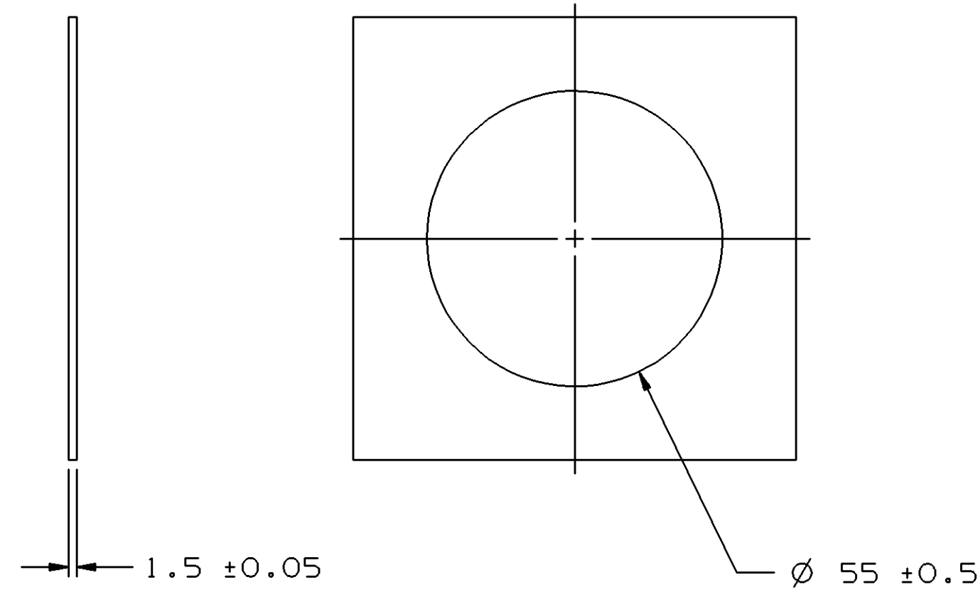
MOUNTING HOLE DETAIL (DOOR)
