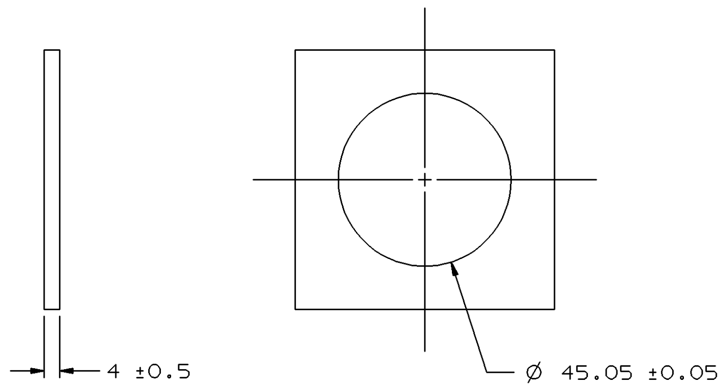
MOUNTING HOLE DETAIL (PILLAR)
