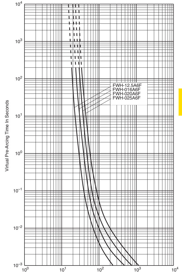
Time-Current Curve
