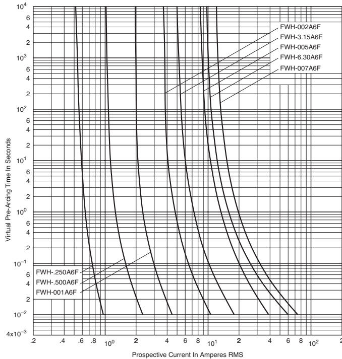
Time-Current Curve
