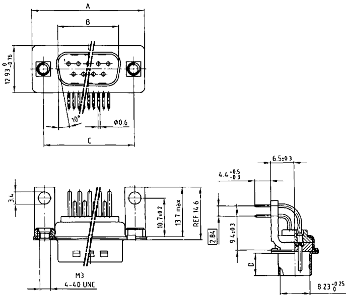
Plug connector
