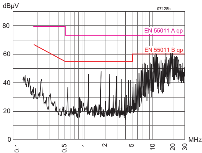
Fig. 21a BP 2320-9RD Typ. conducted disturbance voltage at the input ( V_{i nom} , I_{i nom} , resistive load, quasi peak).
