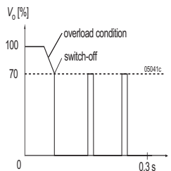
Fig. 8 Overload switch-off (hiccup mode); typical values
