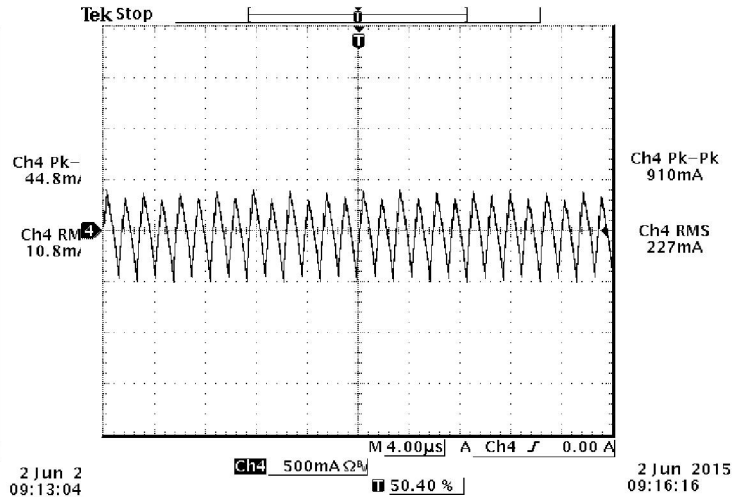
ic (input terminal ripple current), AC component
