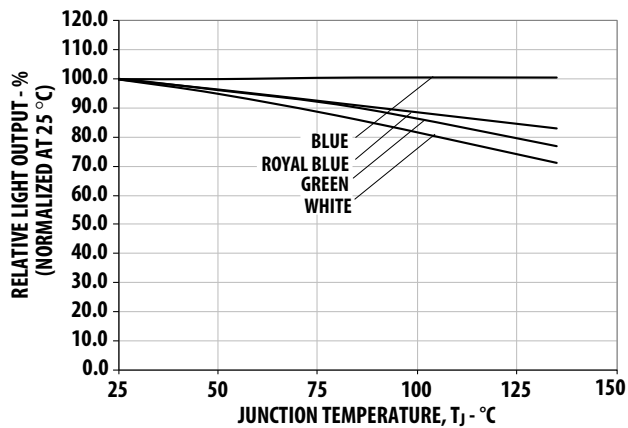
Figure 23 Relative Light Output vs. Junction Temperature
