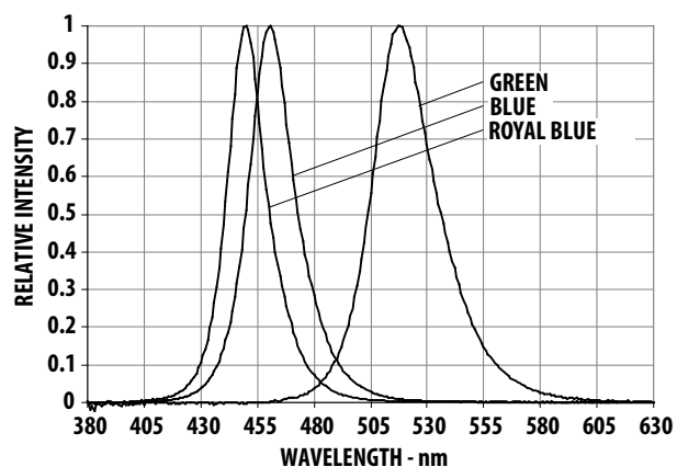
Figure 16 Relative Intensity vs. Wavelength for Blue, Royal Blue and Green
