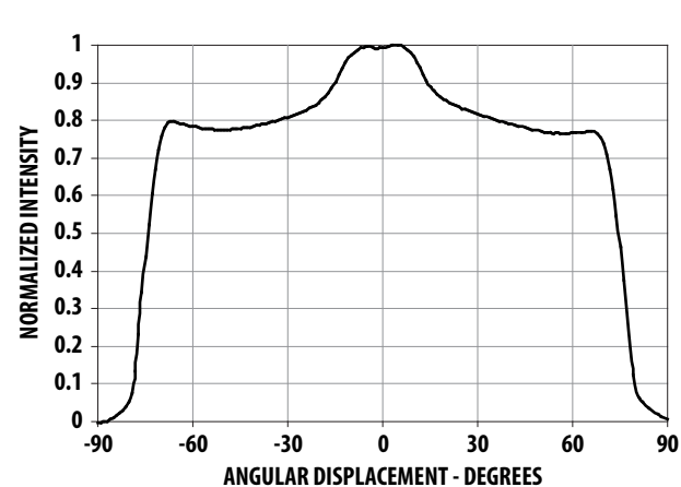
Figure 8 Radiation Pattern for Red, Red Orange, and Amber
