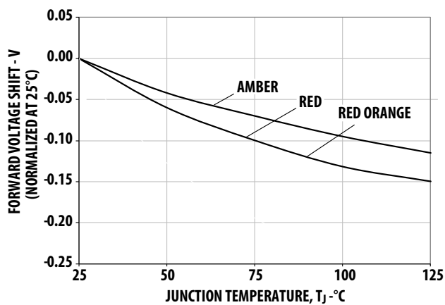
Figure 12 Forward Voltage Shift vs. Junction Temperature
