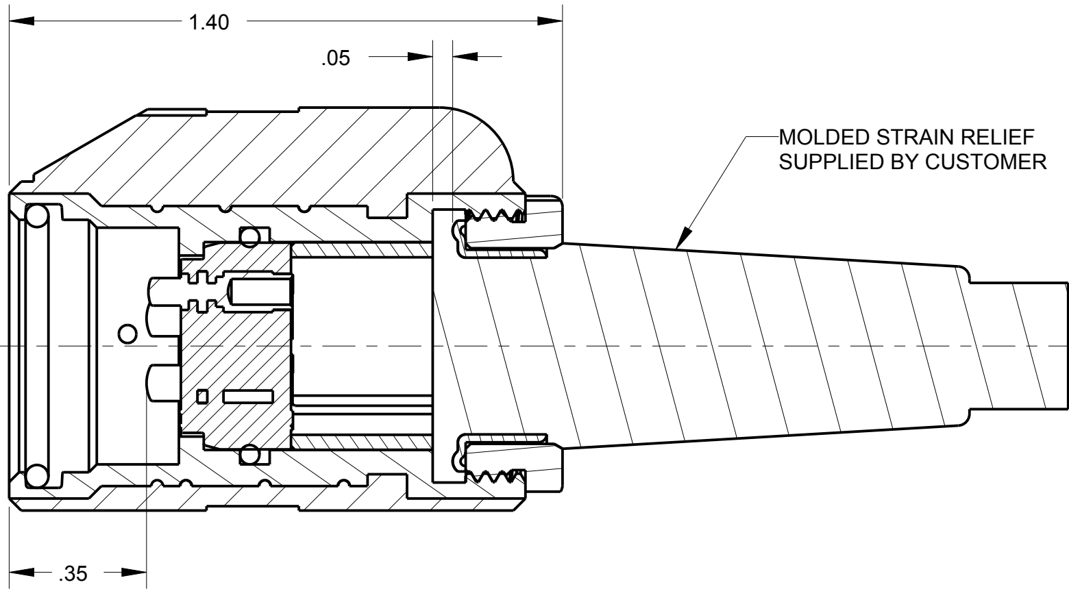
SECTION Z-Z
