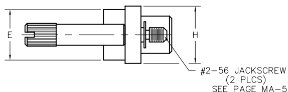
PLUG
