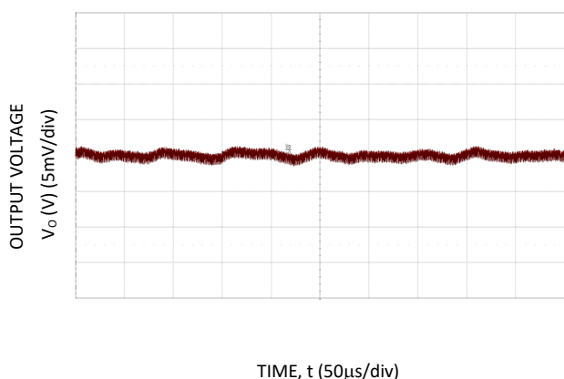
Figure 9. Typical output ripple and noise ( C_o=12 \times 47\mu\text{F} ceramic + 10 \times 470\mu\text{F} polymer, V_{IN} = 12\text{V} , I_o = I_{o,max} )
