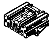
7198-1706-30 ISOMETRIC VIEW (SCALE 1:1)
