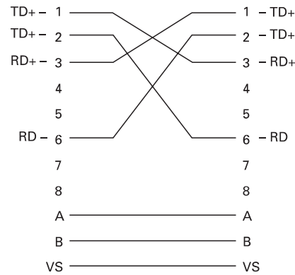
Wiring Diagram for Y-ConJack-25
