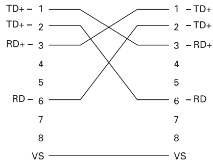
Wiring Diagram for Y-ConJack-15
