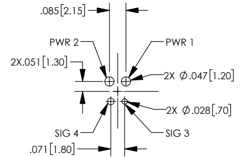
RECOMMENDED FOOTPRINT
