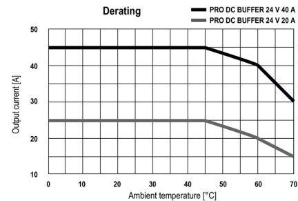
Temperature Derating
