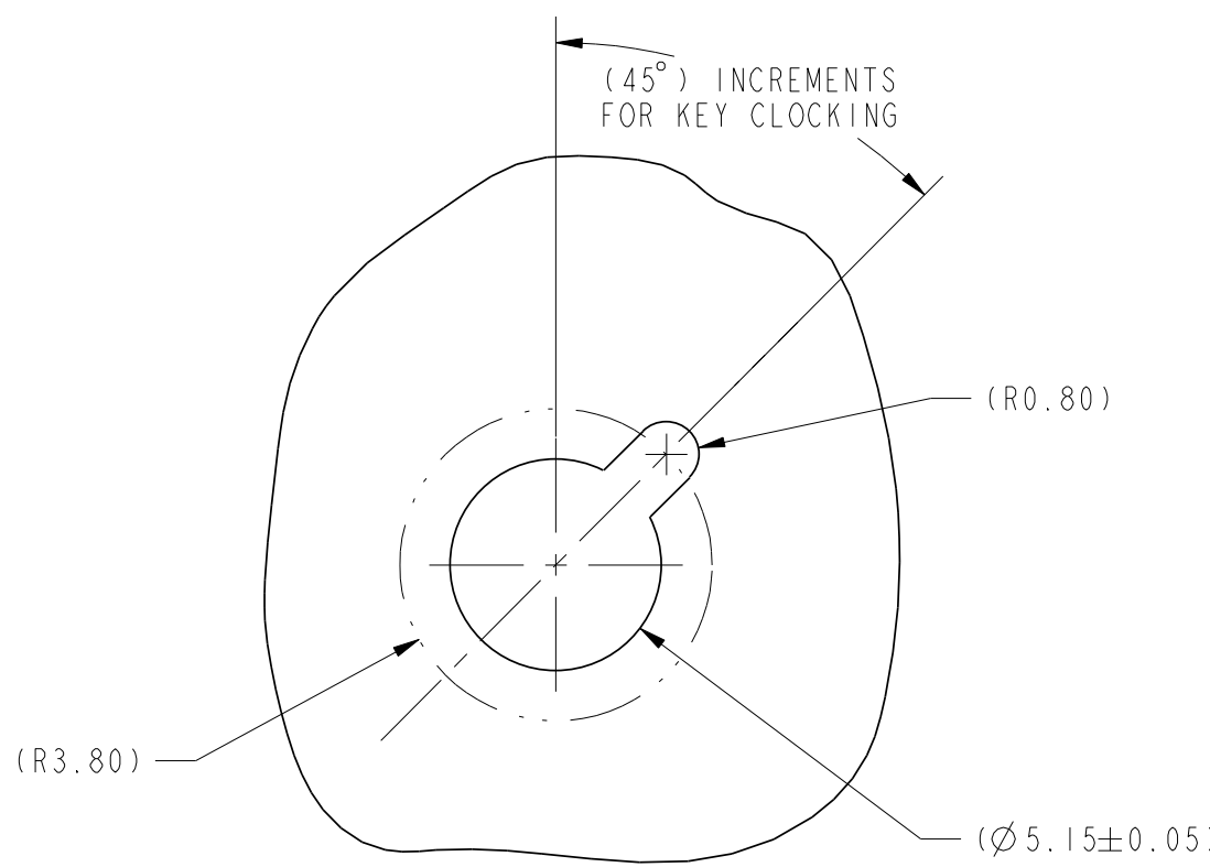
DETAIL A (4) 2 PLACES SCALE 5/1 OPTIONAL HOLE CONFIGURATION NOT REQUIRED FOR AMPHENOL PRODUCT
