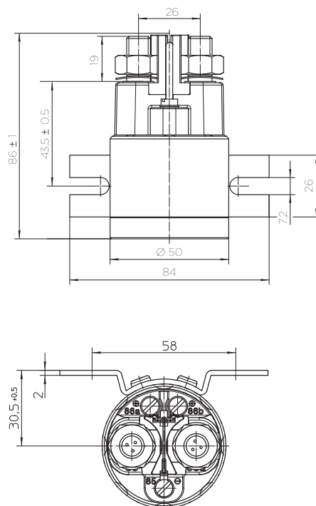
Long form side mounting
