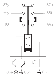
NO-Contact Auxiliary contact / Magnetic blowout
