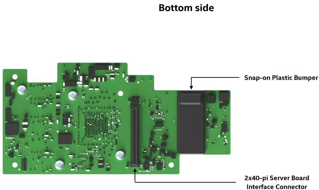
Figure 1. Intel® RMSP3JD160F Storage Module layout
