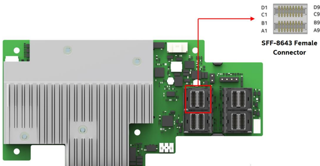
Figure 5. Intel® RMSP3JD160F RAID Module SFF-8643 connector
