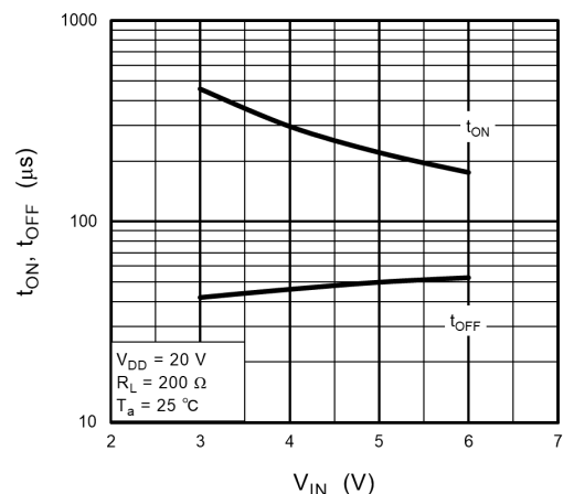
Fig. 12.6 t_{ON}, t_{OFF} - V_{IN}
