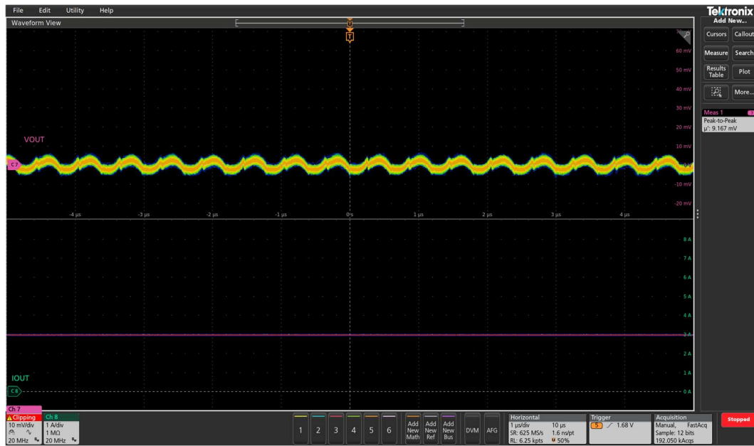
Figure 18 V_{OUT} ripple at 3A (Ch7: V_{OUT} , Ch8: I_{OUT} ), Peak-Peak V_{OUT} ripple = 9.17mV
