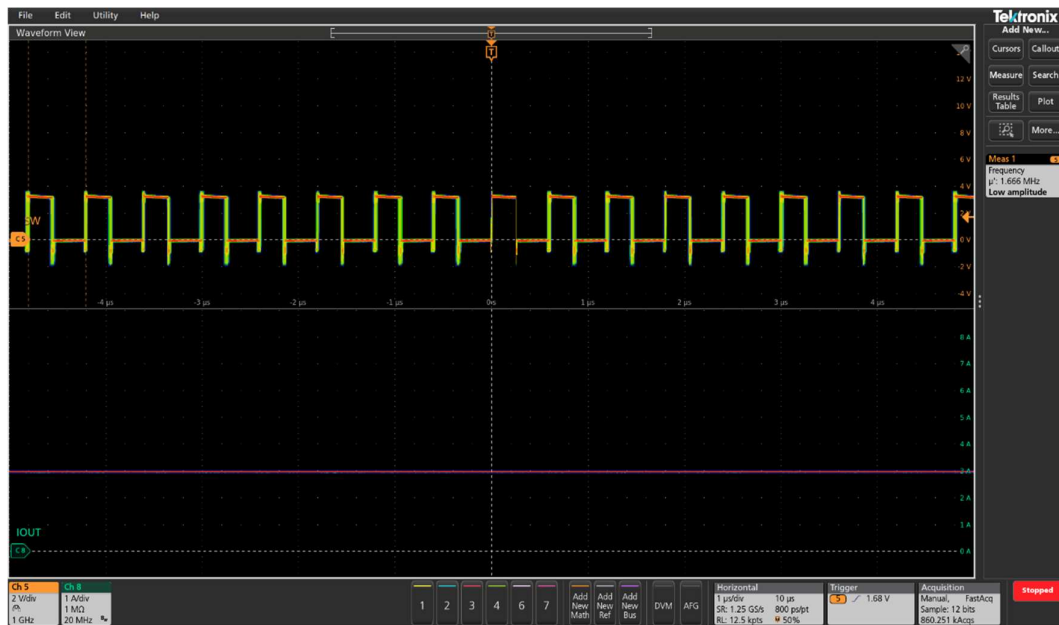
Figure 16 Sw at 3A (Ch5: Sw, Ch8: IOUT), F_{SW} = 1.67\text{MHz}
