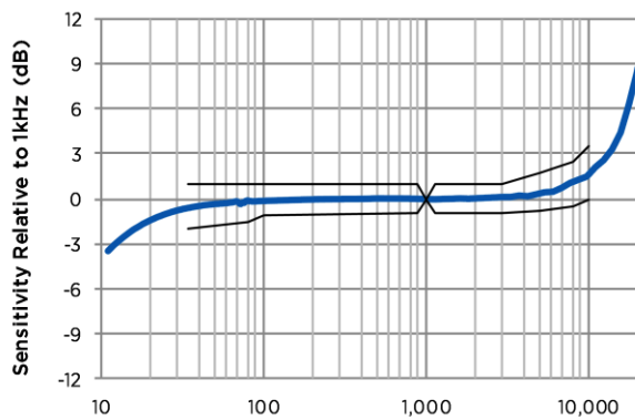
Figure 1: Typical Free Field Magnitude Response and Masks
