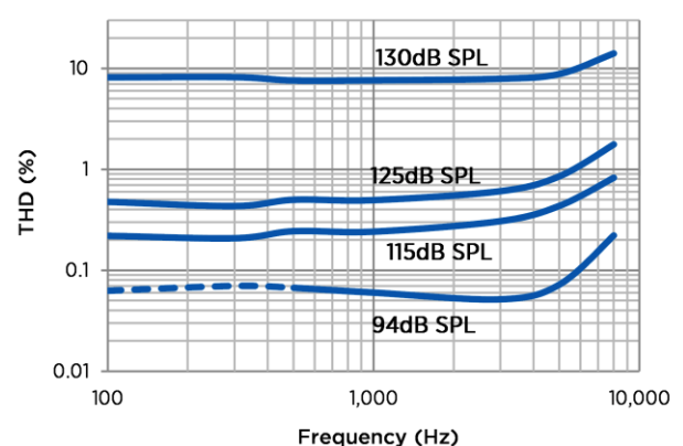
Figure 4: Typical THD vs Frequency
