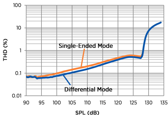
Figure 2: Typical THD vs SPL
