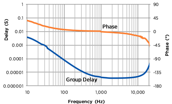
Figure 3: Typical Phase and Group Delay
