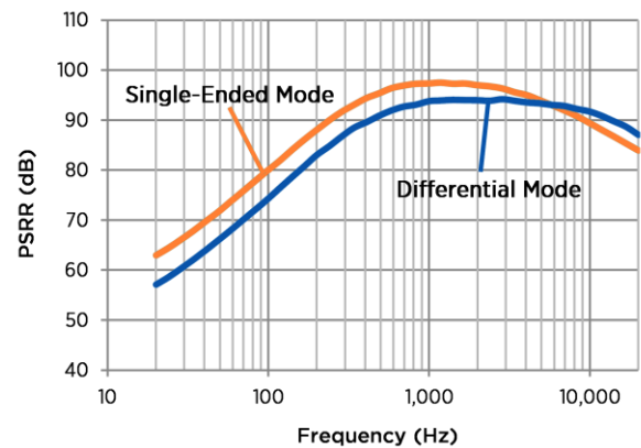
Figure 8: Typical PSRR
