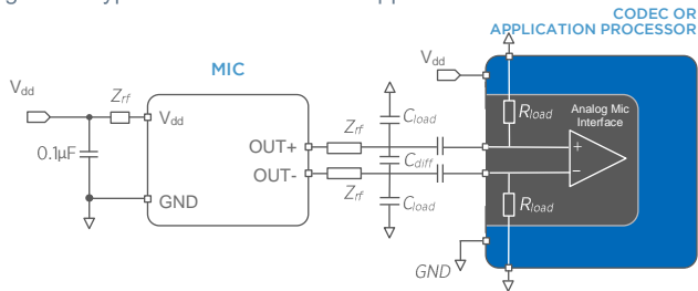
Figure 1: Typical Differential Mode Application Circuit
