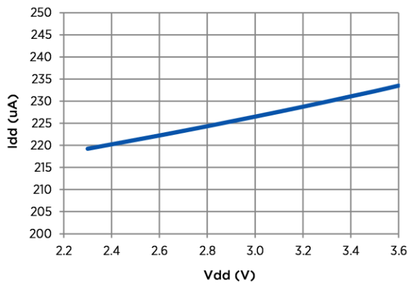
Figure 6: Typical I_{dd} vs V_{dd}
