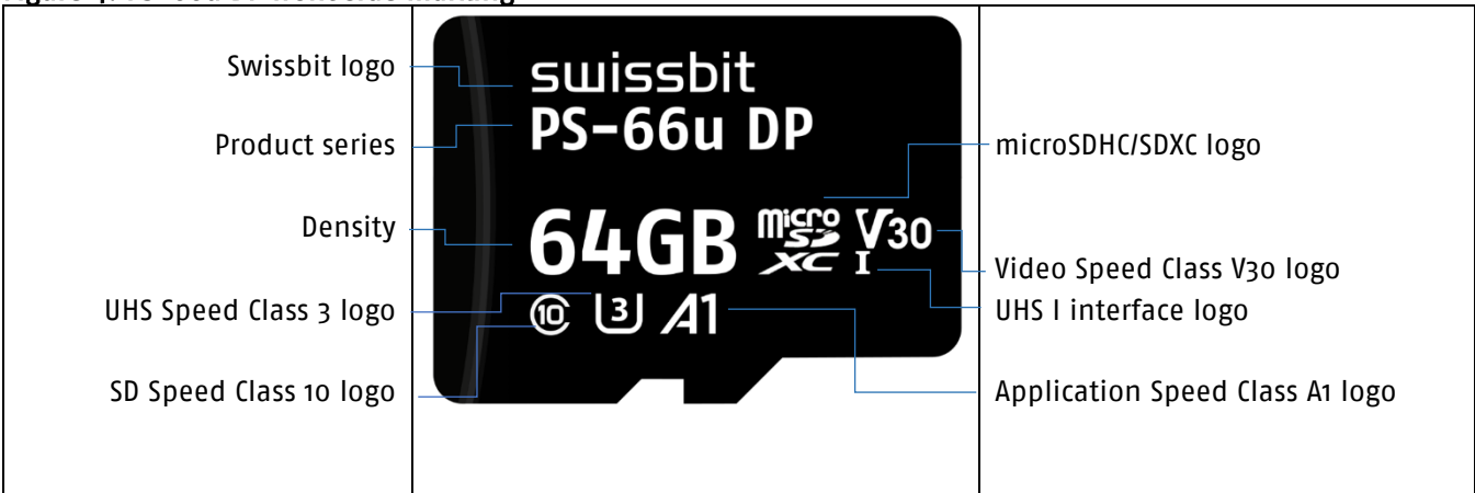
Figure 4: PS-66u DP front side marking
