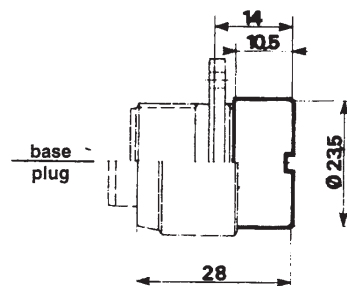
Backnut
