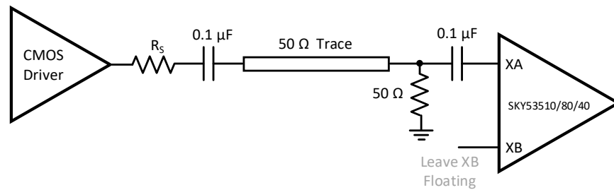
Figure 17. Driving XA with a Single-Ended Input Clock
