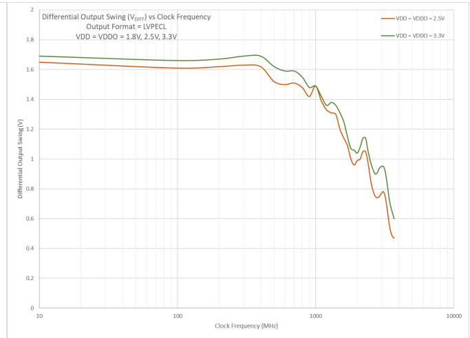
Figure 46. Differential Output Voltage Swing vs. Frequency (2.5 V, 3.3 V LVPECL)
