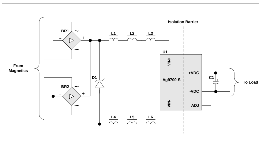
Figure 19: EMC Filtering
