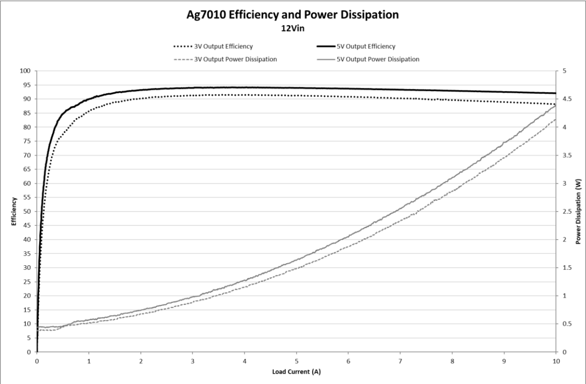
Figure 5: Ag7010 Efficiency with 12V Supply
