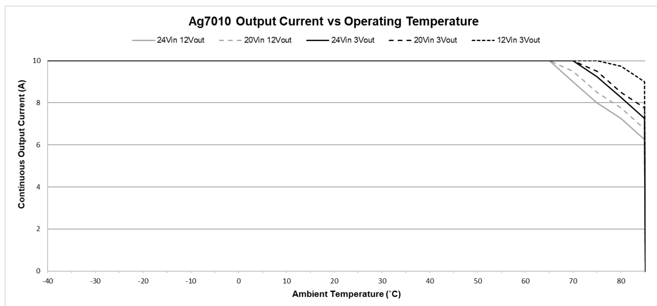
Figure 11: Ag7010 operating temperature profile
