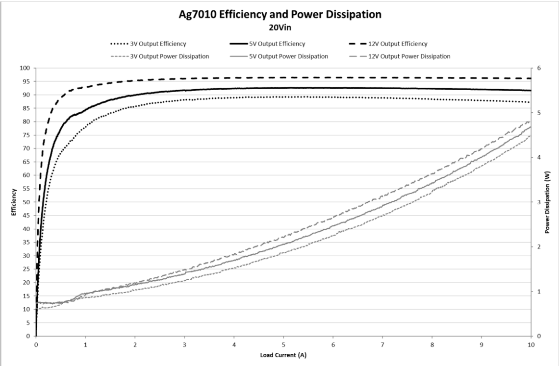
Figure 6: Ag7010 Efficiency with 20V Supply
