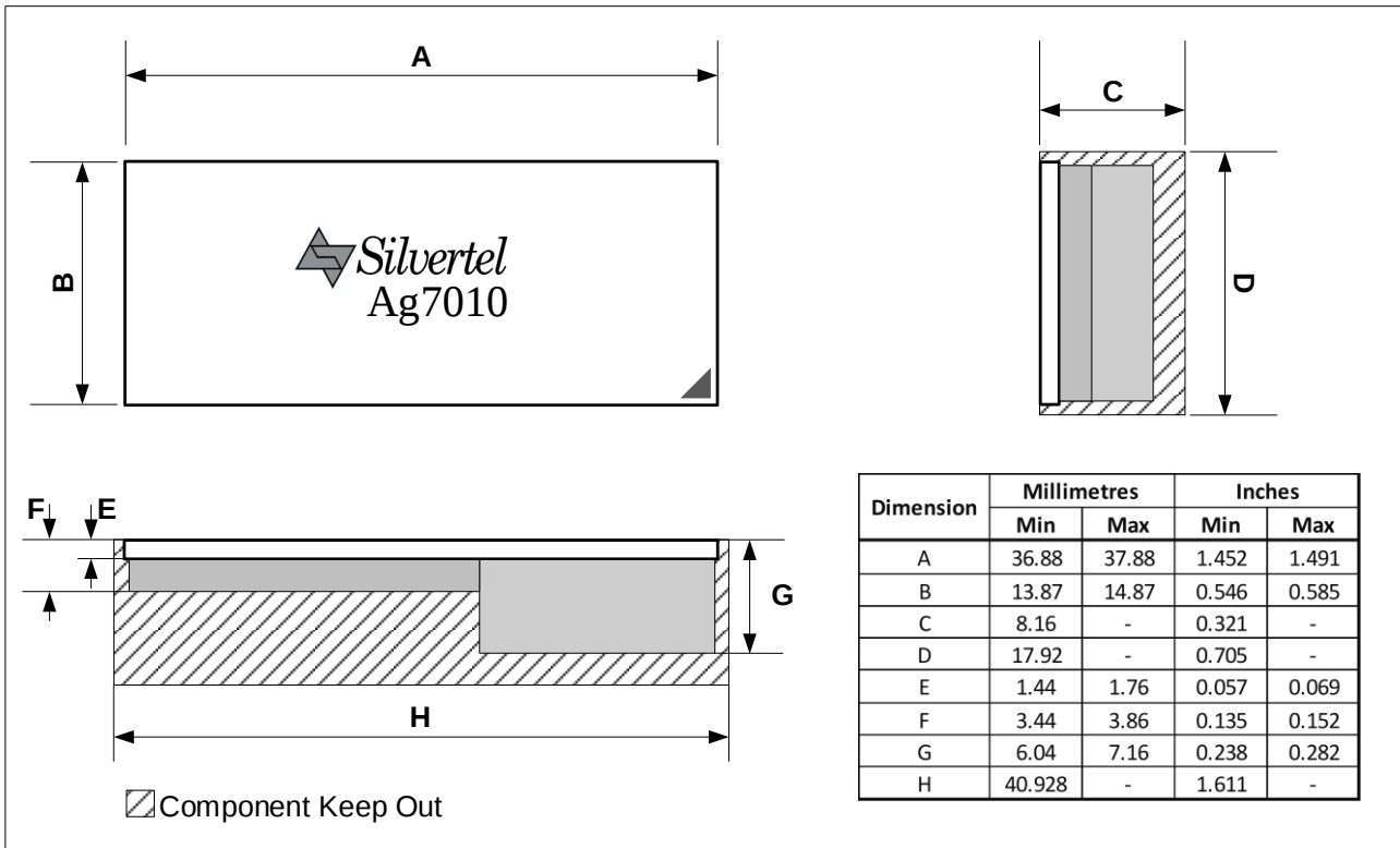
Figure 15: Package Dimensions
