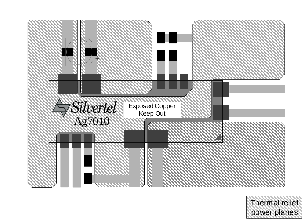
Figure 12: Thermal Relief
