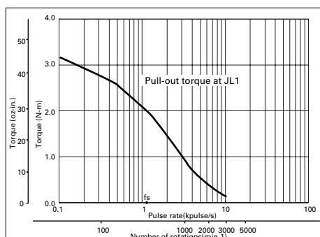
SM2861-5052(Single shaft) SM2861-5022(Double shaft) Input current: 2A/phase
