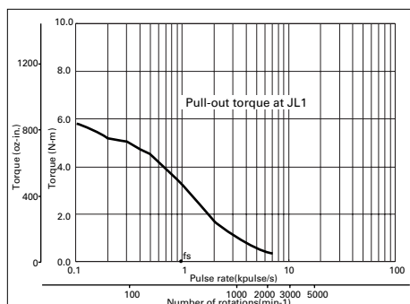
SM2863-5052(Single shaft) SM2863-5022(Double shaft) Input current: 2A/phase
