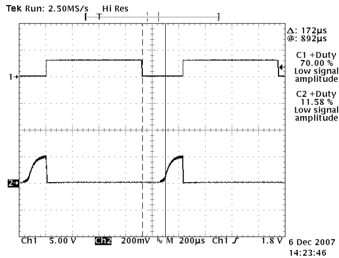
Figure 3. 1KHz, 70% duty cycle dimming signal is approximately 10% LED duty cycle Ch1 = DIM signal, Ch2 = VFB 200mV/div = 2A Output current/div
