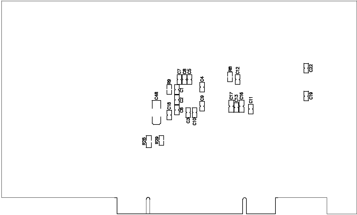
Figure 10-2: S5U13A05P00C100 Board Layout (Bottom View)
