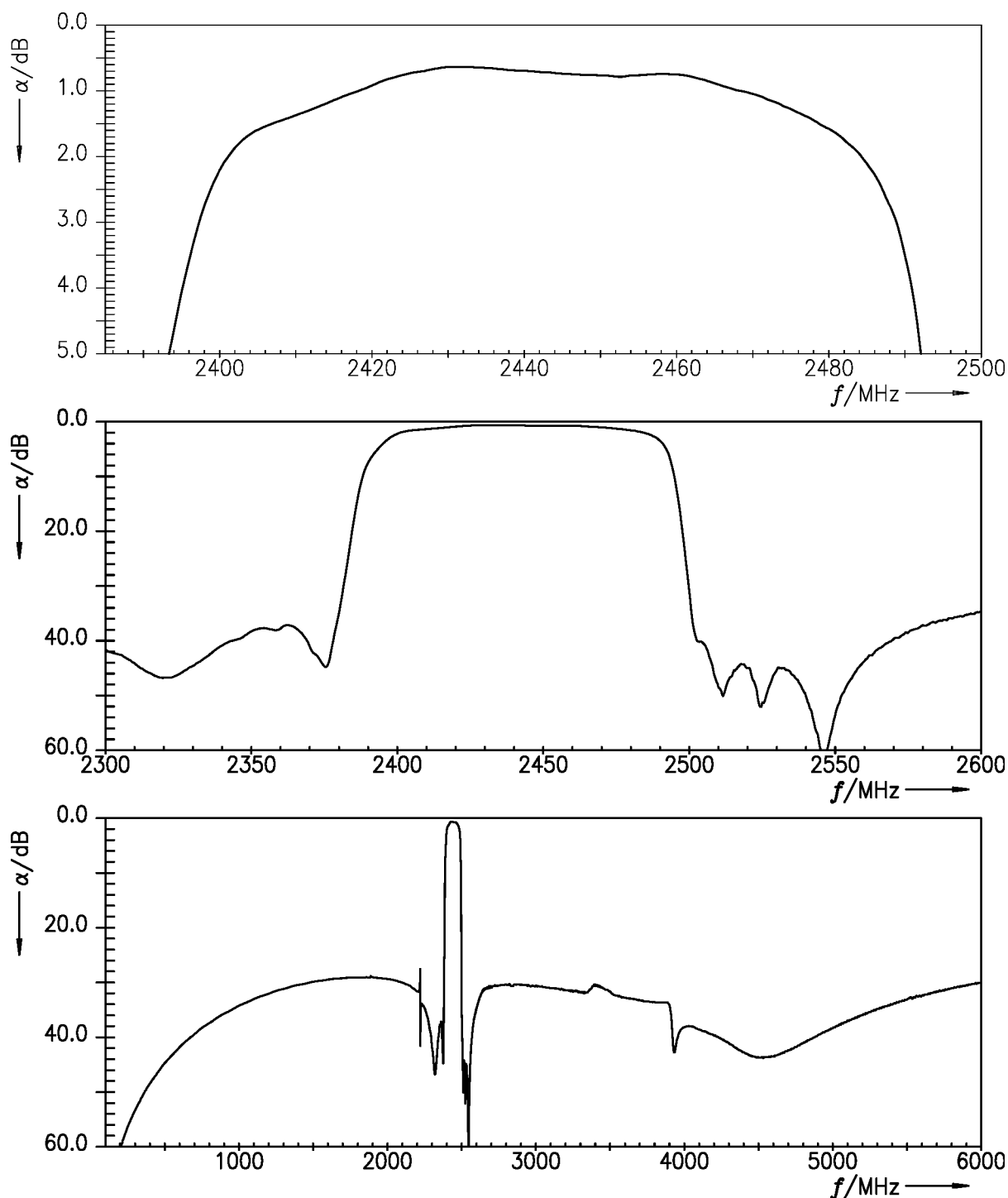
Figure 4: Attenuation.
