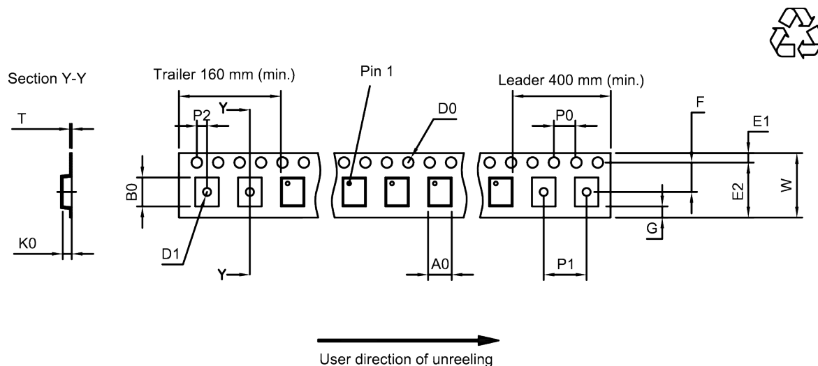
Figure 7: Drawing of tape (first-angle projection) is for illustration only and not to scale. Tape Dimensions in Table 1 are the valid dimensions for the tape.
