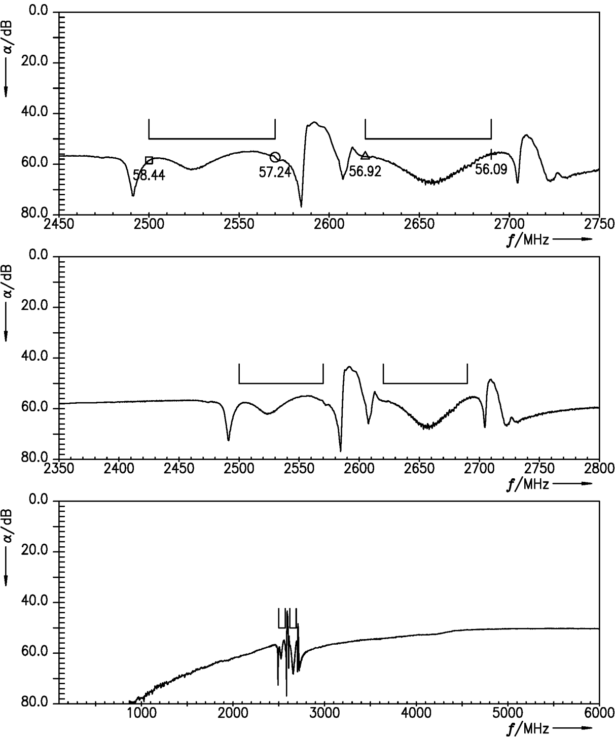
Figure 6: Isolation RX – TX.
