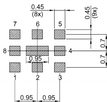
Figure 2: Drawing of package with package height A = 0.5 mm (max.). See Sec. Package information (p. 22).
